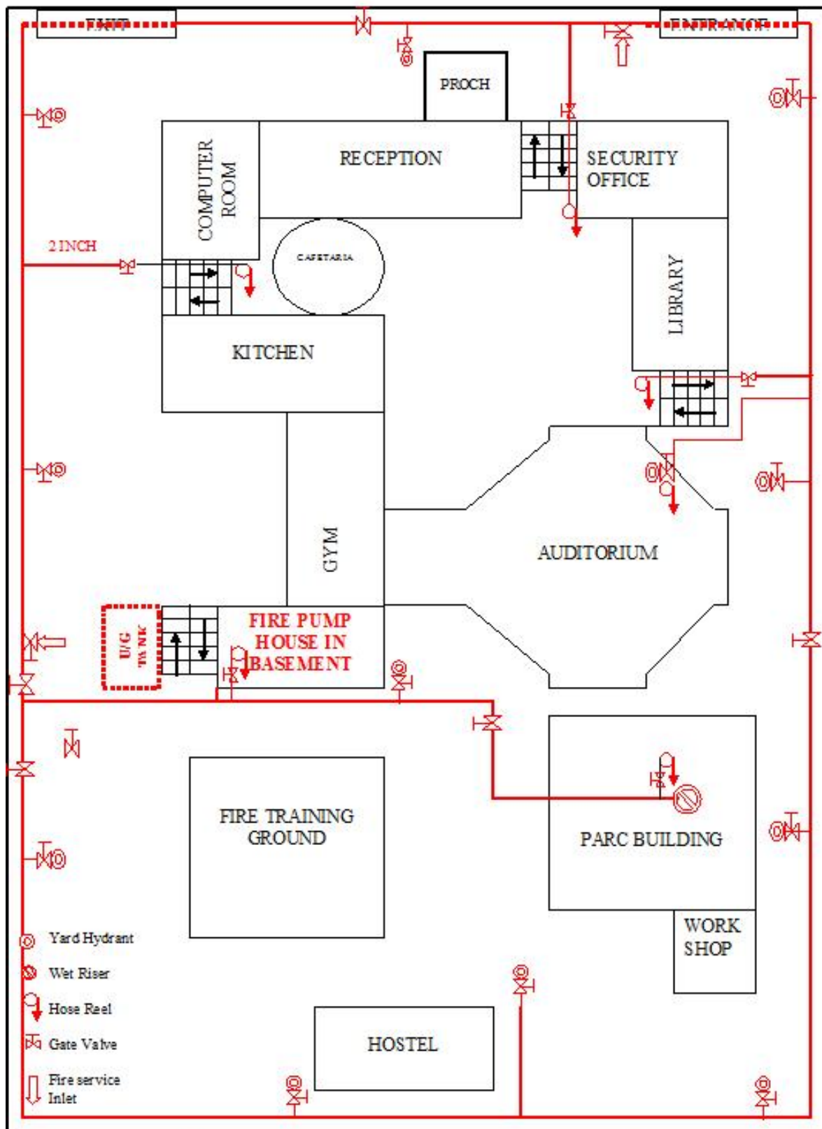
SKETCH FOR INTENDED FIRE WATER NETWORK LAYOUT AT GTI COMPLEX
