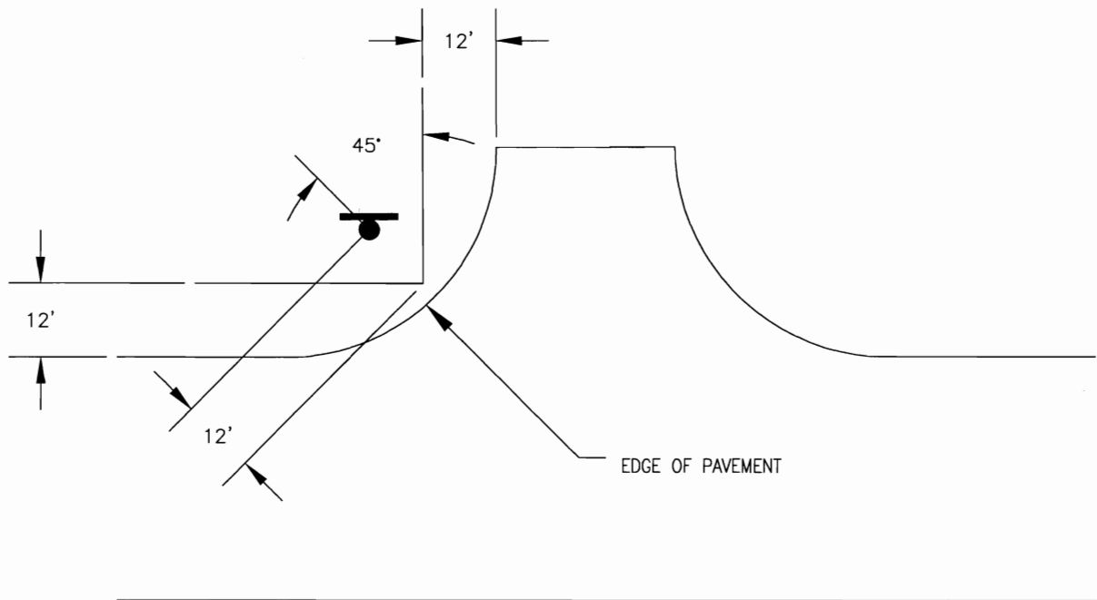
STOP SIGN PLACEMENT DETAIL
