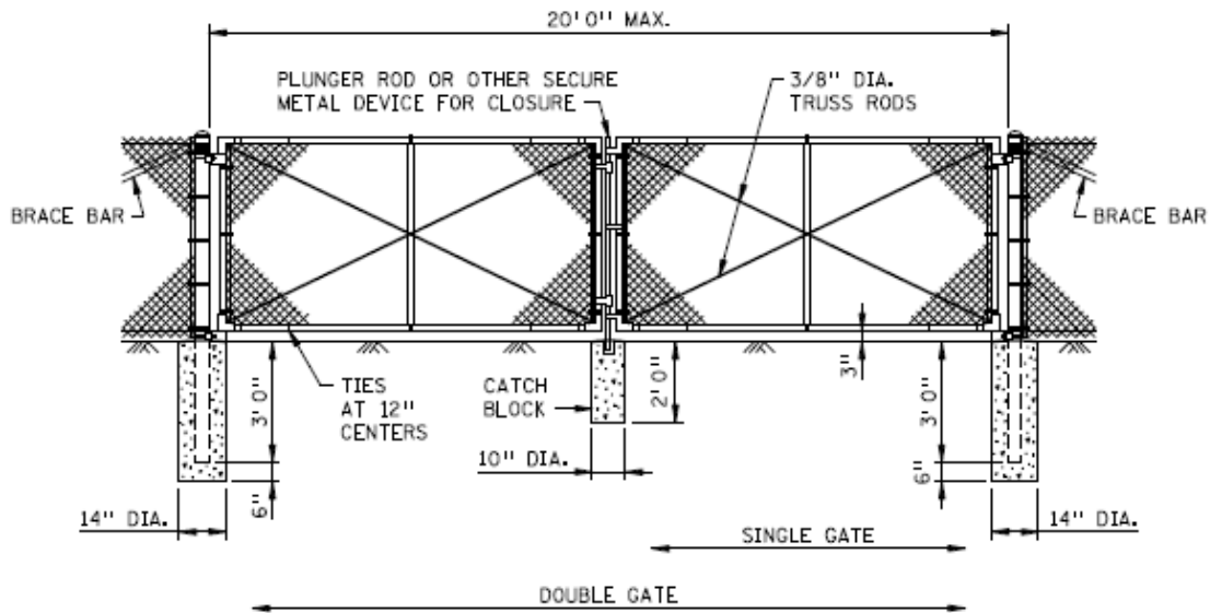
VEHICULAR GATE
