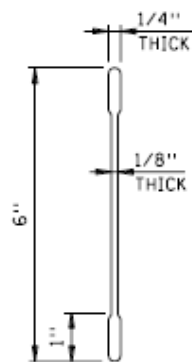
SECTION ALUMINUM BASE PLATE
