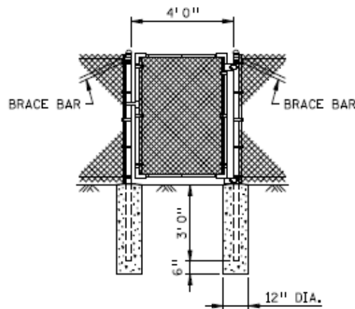
PEDESTRIAN GATE
