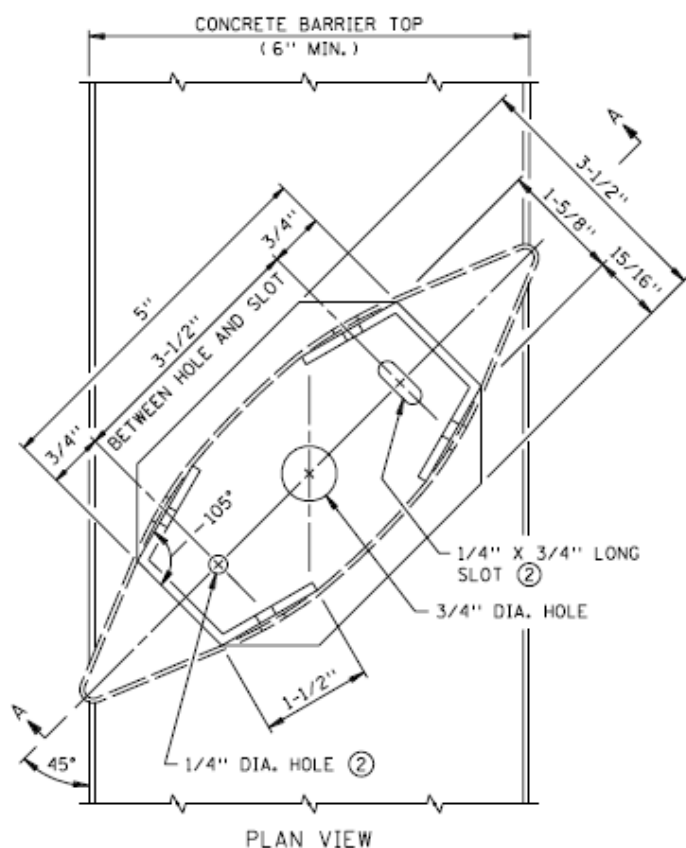
PLAN VIEW
